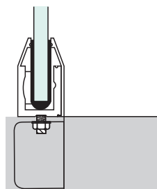
M10 at 400 ctc Bolt
