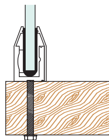
M10 at 200 ctc Bolt
