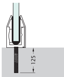
M10 at 200 ctc chemset
