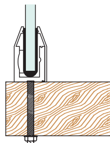
M10 at 200 ctc Bolt
