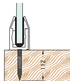
M10 at 200 ctc Coach Screw
