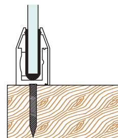
Internal M10x95mm at 200ctc Eternal M10x112mm at 200ctc
